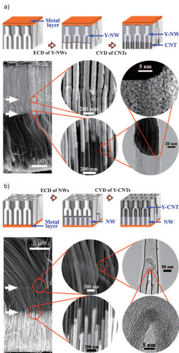
Figure 2. Two types of mirrored NT/NW hybrid architectures with Y-branched topology. a) Y-NiNW/2CNTs hybrid structure. One Y-shaped NiNW connects with two parallel CNTs in the branches of the Y construct. b) Y-CNT/2NiNWs hybrid structure. One Y-CNT connects with two parallel NiNWs in the branches of the Y construct. The upper panels are schematic drawings depicting three characteristic moments of the fabrication procedure, in which the planar surface of the stem-channel side (a) or branched-channel side (b) of the Y-AAO templates is coated with a thin metal layer as electrode in the ECD of NiNWs. The lower panels on the left are scanning electron microscopy (SEM) images of a bundle of the structures after template removal, in which the light and dark parts are NiNWs and CNTs, respectively; the two parallel interfaces (white arrows) show Y branchings and NiNW/CNT junctions. The lower middle panels are close-up views of the Y branchings (top) and NiNW/CNT junctions (bottom). The lower right panels are TEM (top) and high-resolution TEM images (bottom) of a NiNW/CNT junction (a) and a Y-CNT (b).
